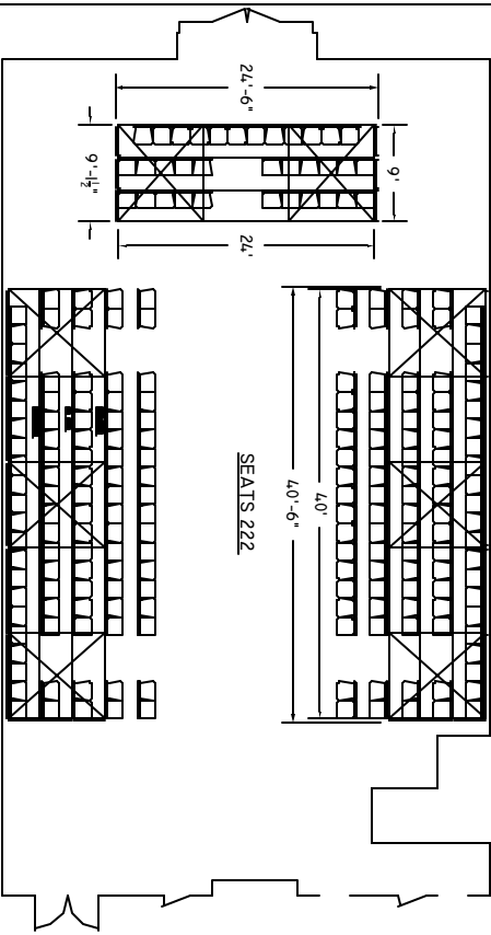
RISER PLAN VIEW LAYOUT #3
